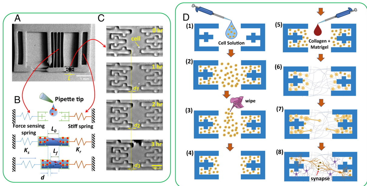
Fig. 1. Schematic representation of the concept and methodology to measure neuronal force using the ultrasensitive force sensor. (A) SEM image of the force sensor. (B) The simplified view of neuronal force measurement technique in a 3D matrix [adapted from Emon et al. (30)]. (C) Bright-field image of the sensor at different time points of culture explaining the force measurement methodology. The left grip is attached to the force sensing spring, and the right grip is attached to the stiff spring. Force produced by the tissue at any time t is given by F(t) = K_s \cdot d(t) , where K_s and d(t) refer to the stiffness and the displacement at any time point for the force-sensing spring, respectively. As time progresses, there is an evident increase in the displacement of the force-sensing grip, suggesting a rise in force over time (see Movie S3 for the full time-lapse video). (D) The schematic diagram of the steps to form the 3D neuronal tissue (created with BioRender.com ).
