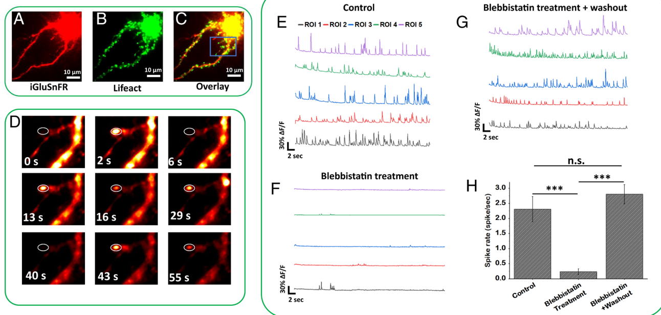
Fig. 6. Force disruption using blebbistatin significantly decreases the neuronal firing at single synapse level which is recoverable after drug washout; Rat hippocampal neurons cotransfected with (A) iGluSnFR and (B) Lifeact-miRFP. (C) Overlay image of iGluSnFR and Lifeact-miRFP showing the dendritic spine along the length of neurite. (D) Time series image of a single synapse (labeled by a white oval) showing the variation of iGluSnFR intensity at different time points. Time history of firing pattern at the individual synapse of neuronal culture from (E) control group. (F) Blebbistatin treatment. (G) Blebbistatin treatment with the washout group. (H) Spike rate at the individual synapse for the neuronal culture of different groups ( n = 3 ). The chart shows mean \pm SEM. Statistical significance was determined using one-sided ANOVA with Tukey test; n.s., not significant; * P < 0.05 ; ** P < 0.001 ; and *** P < 0.0001 .
